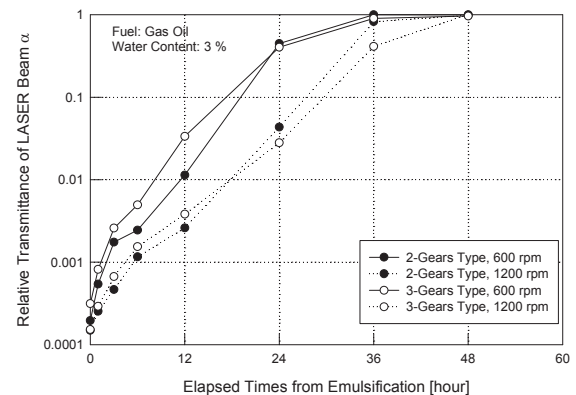
Fig.11 Relative transmittance of laser beam through the emulsified gas oil.
